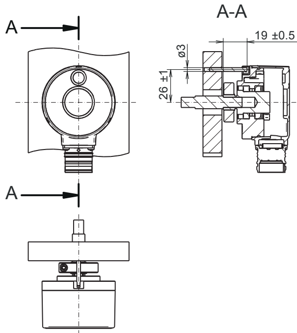
Pin torque support, axial, clamping ring at A-side
