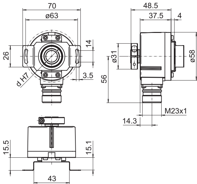
Clamping ring at B-side: Through hollow shaft, flange connector M23 radial
